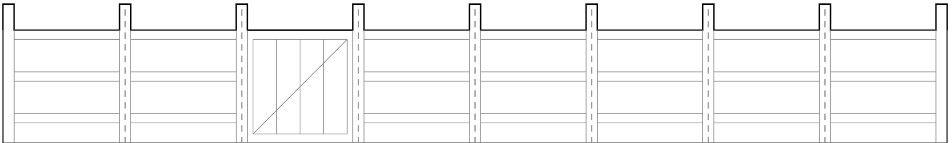
FENCE STRIP 2 — 8 panels, gate is panel 3
